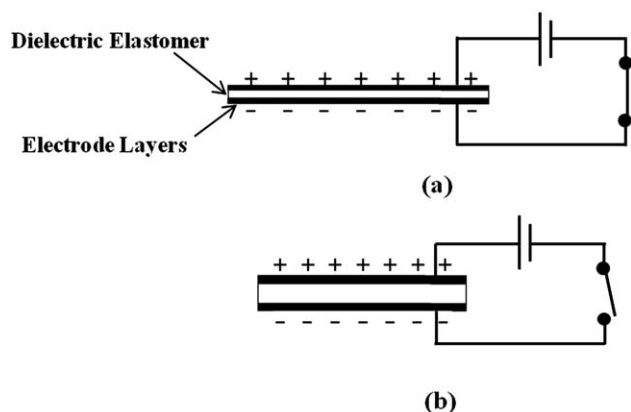
Figure 1. Schematic representation of dielectric elastomer generator (a) at stretched state with low voltage and (b) at relaxed state with high voltage.
